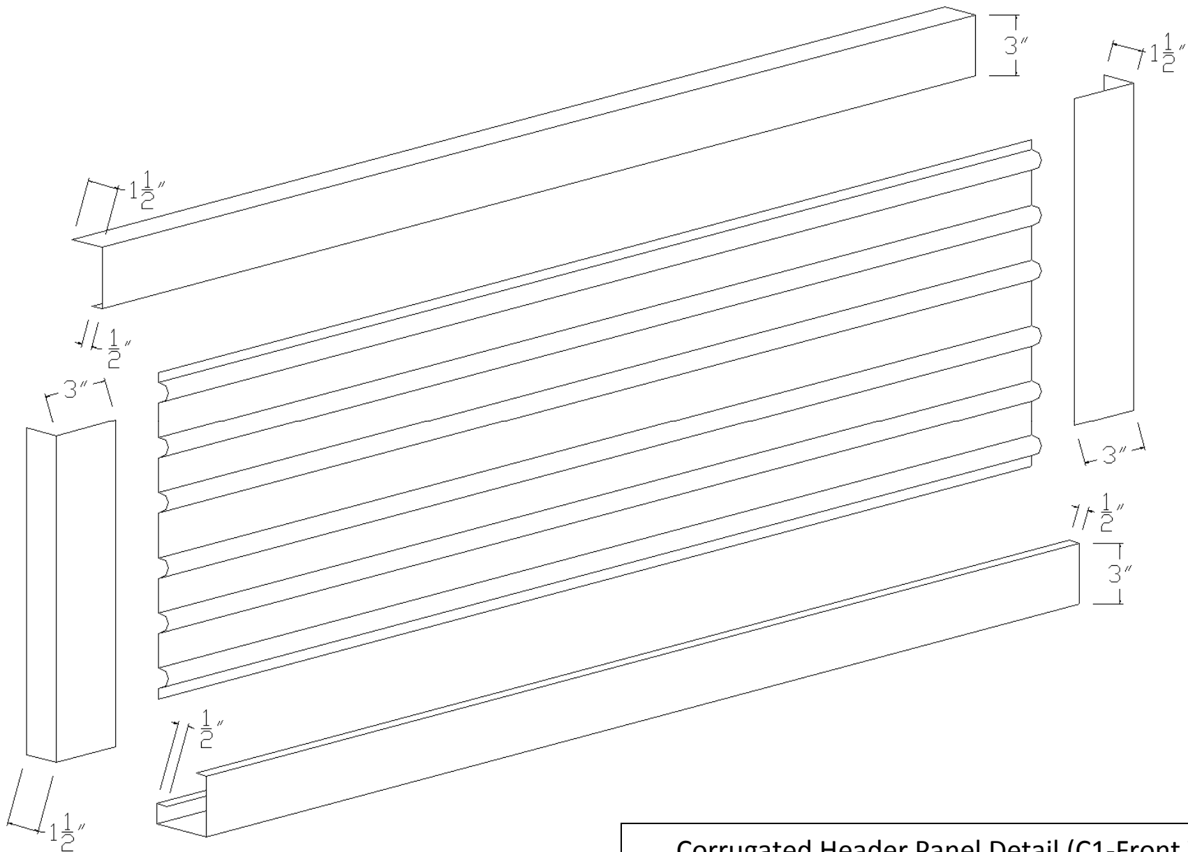
Corrugated Header Panel Detail (C1-Front View)
