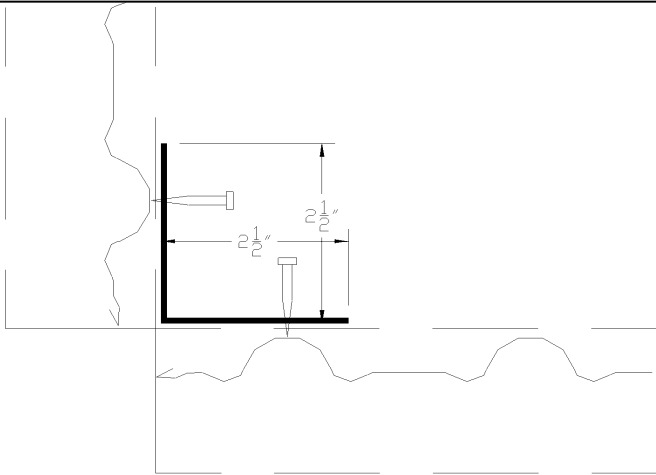
Inside Corner Detail (IS-1)
