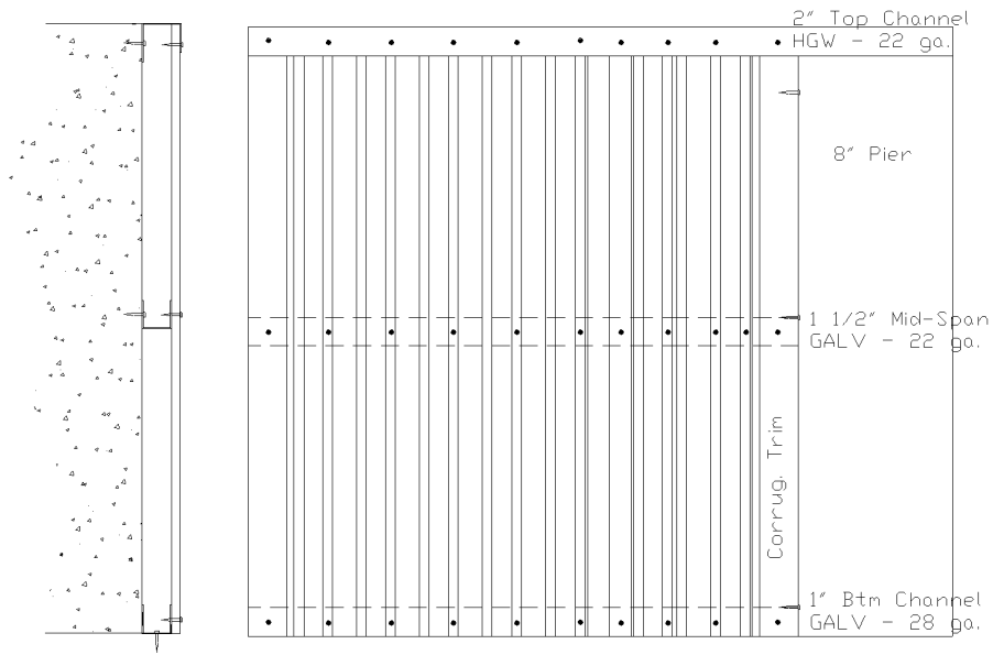
Corrugation Wall Detail (CW-1)
