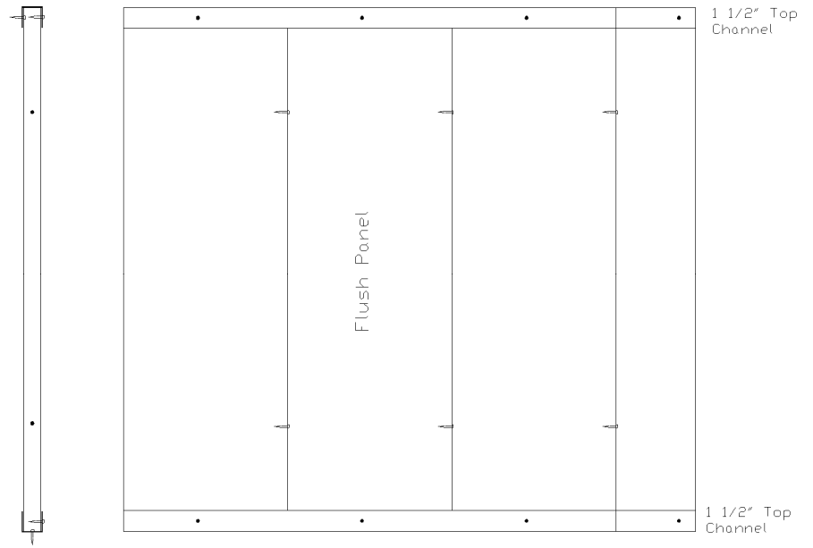
Flush Wall Detail (FW-1)
