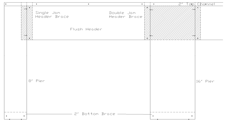
Hallway Detail (H-1)
